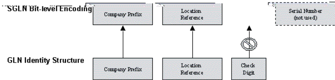
Figure E. How the parts of the decimal SGLN are extracted and rearranged for encoding.
